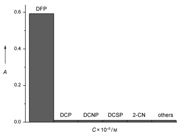
Figure 3. Absorbance at 643 nm (squaraine band) for 1.0 \times 10^{-5} \text{ M} suspensions of N1-1 , SD, and DFP, DCP, DCNP, DCSP, 2-CN, and other guests (1-Ph, DMSP, and 2-oxo) in acetonitrile.
