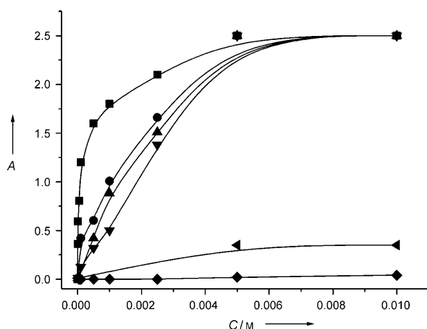
Figure 2. Absorbance at 643 nm (squaraine band) for suspensions of N1-1 , SD, and varying concentrations of DFP (■), DCP (●), DCNP (▲), DCSP (▼), 2-CN (◄), and other species (◆; 1-Ph, DMSP, and 2-oxo) in acetonitrile.
